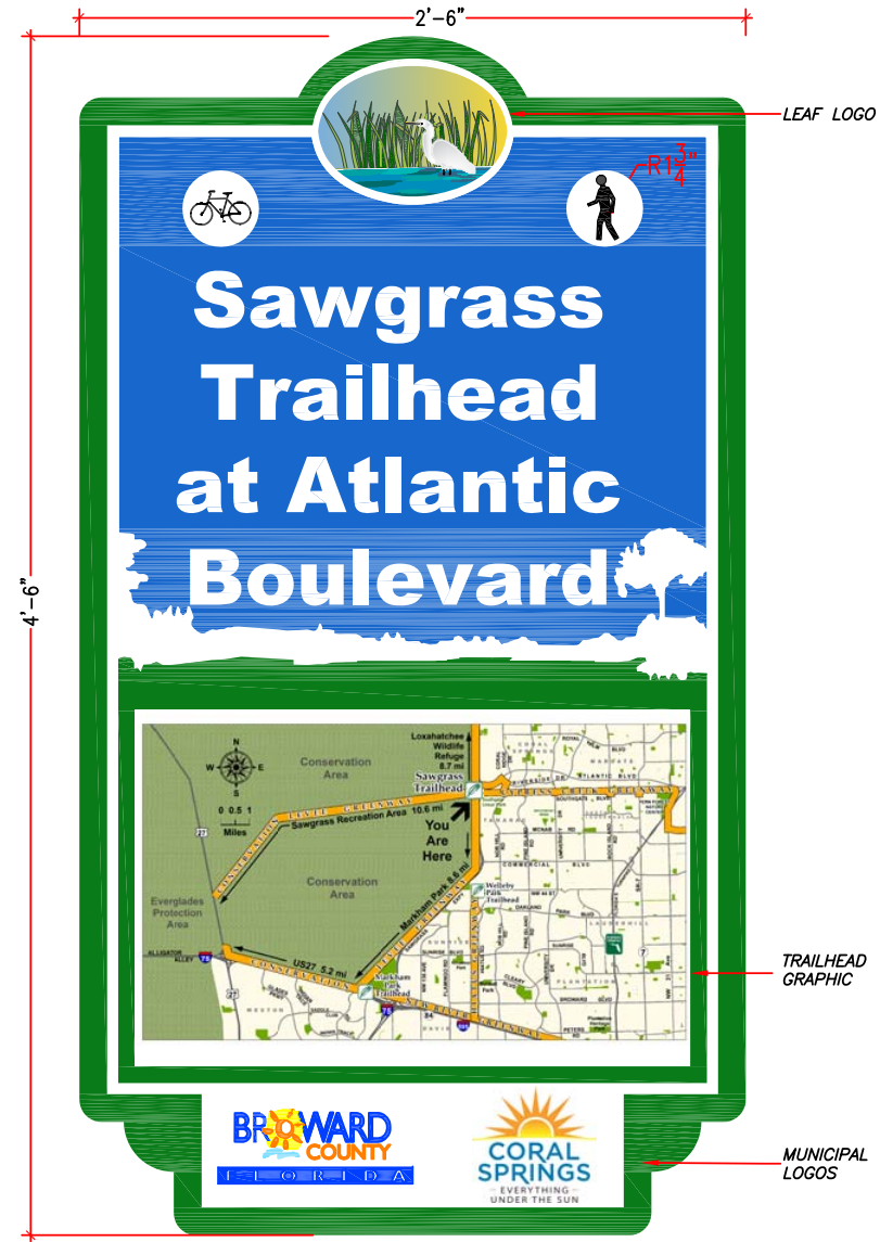
TRAILHEAD SIGN LAYOUT DETAIL N.T.S
