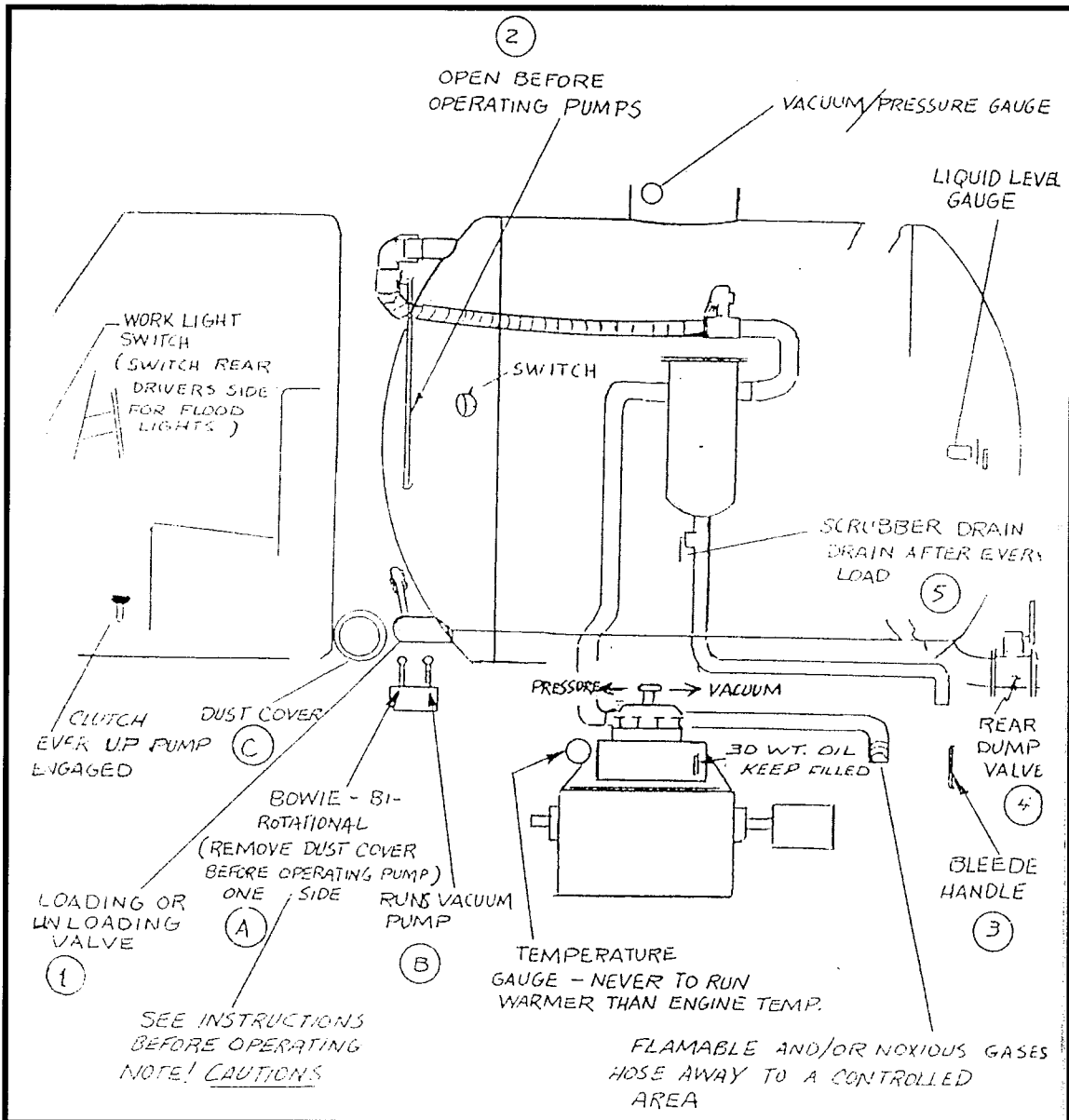
33 CFR 154.310 (a)(2) - Vacuum unit inst 1
