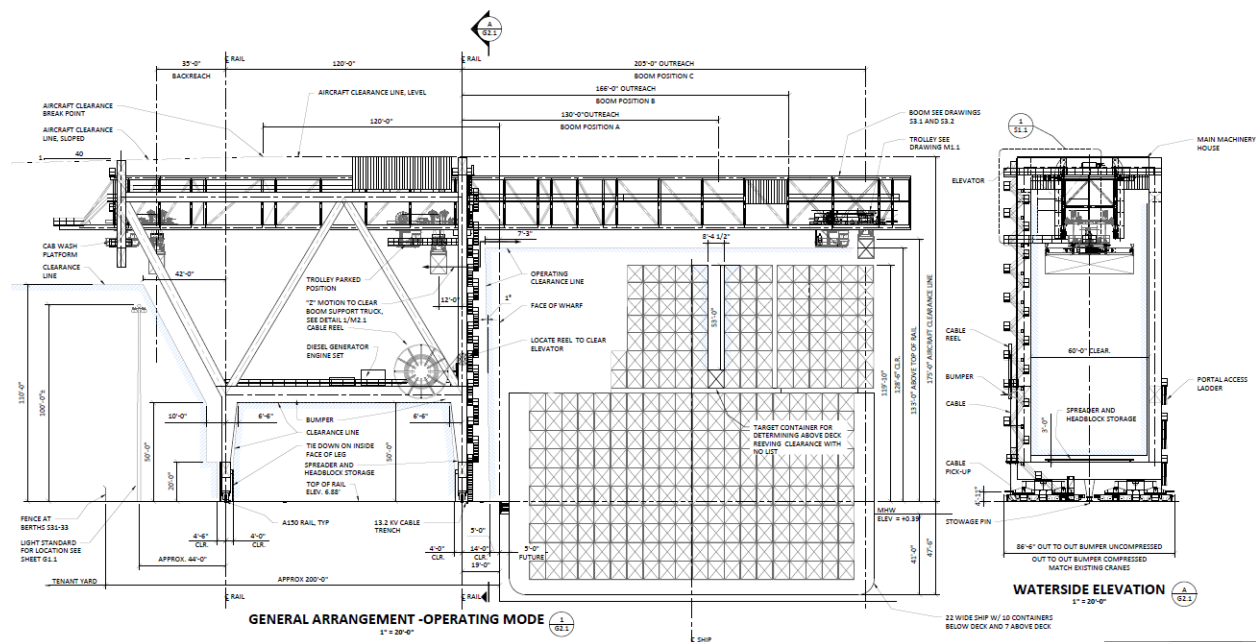
Figure 1: General specifications of Post Panamax Crane
